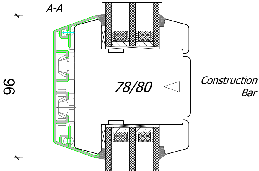
CONSTRUCTION BAR
