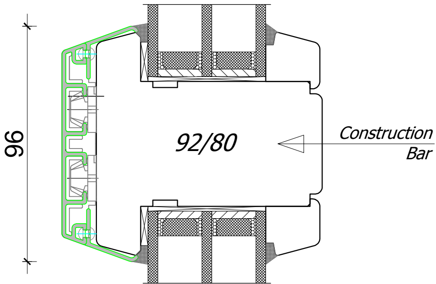
CONSTRUCTION BAR
