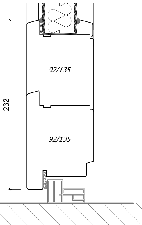
EUROSYSTEM 92 OUTSIDE DOOR OPENING OUTSIDE
