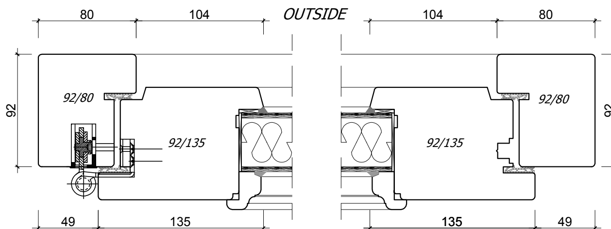
EUROSYSTEM 92 OUTSIDE DOOR OPENING OUTSIDE
