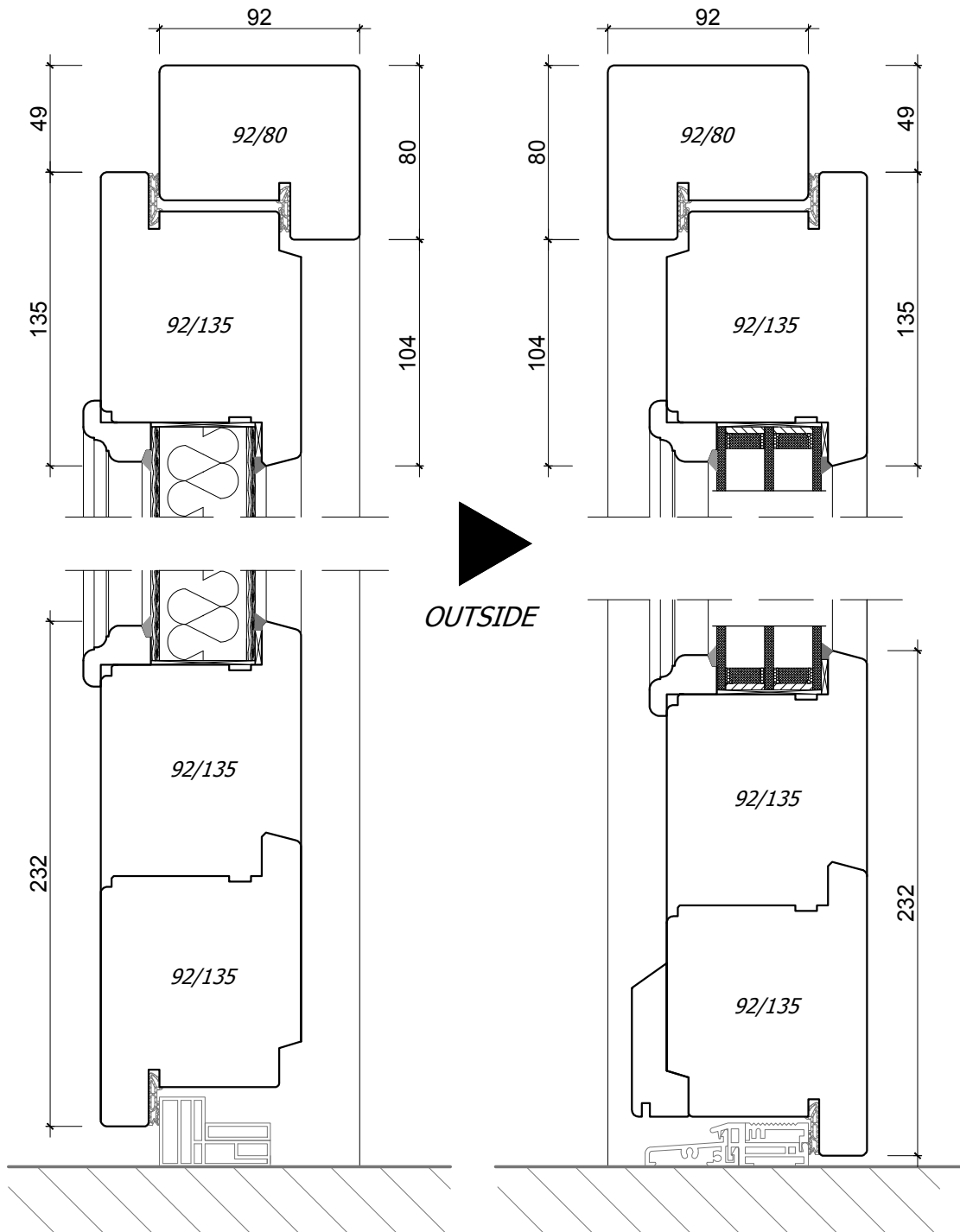
EUROSYSTEM 92 OUTSIDE DOOR OPENING OUTSIDE
