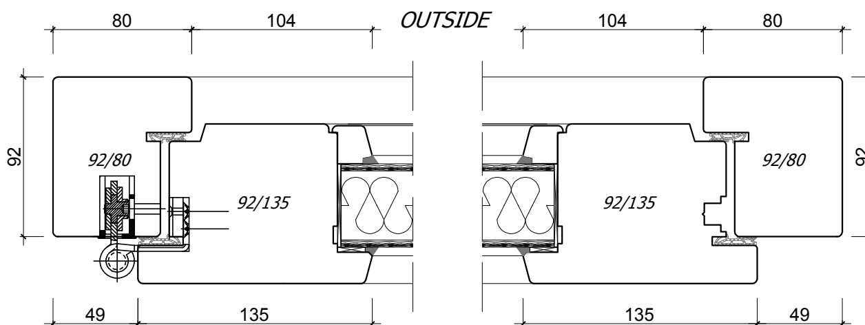
EUROSYSTEM 92 OUTSIDE DOOR OPENING OUTSIDE
