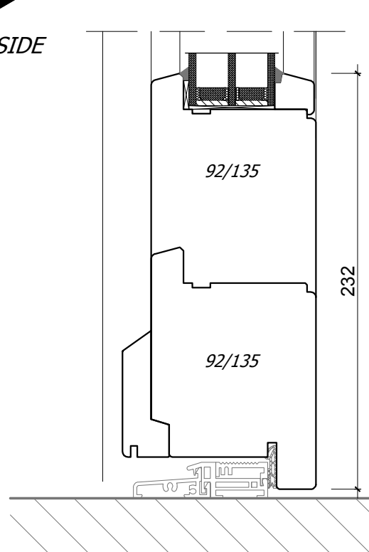
EUROSYSTEM 92 OUTSIDE DOOR OPENING INSIDE
